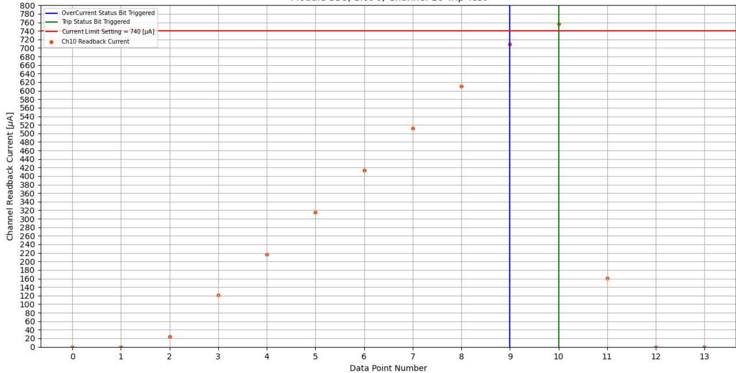
Module 358, Slot 6, Channel 10 Trip Test
