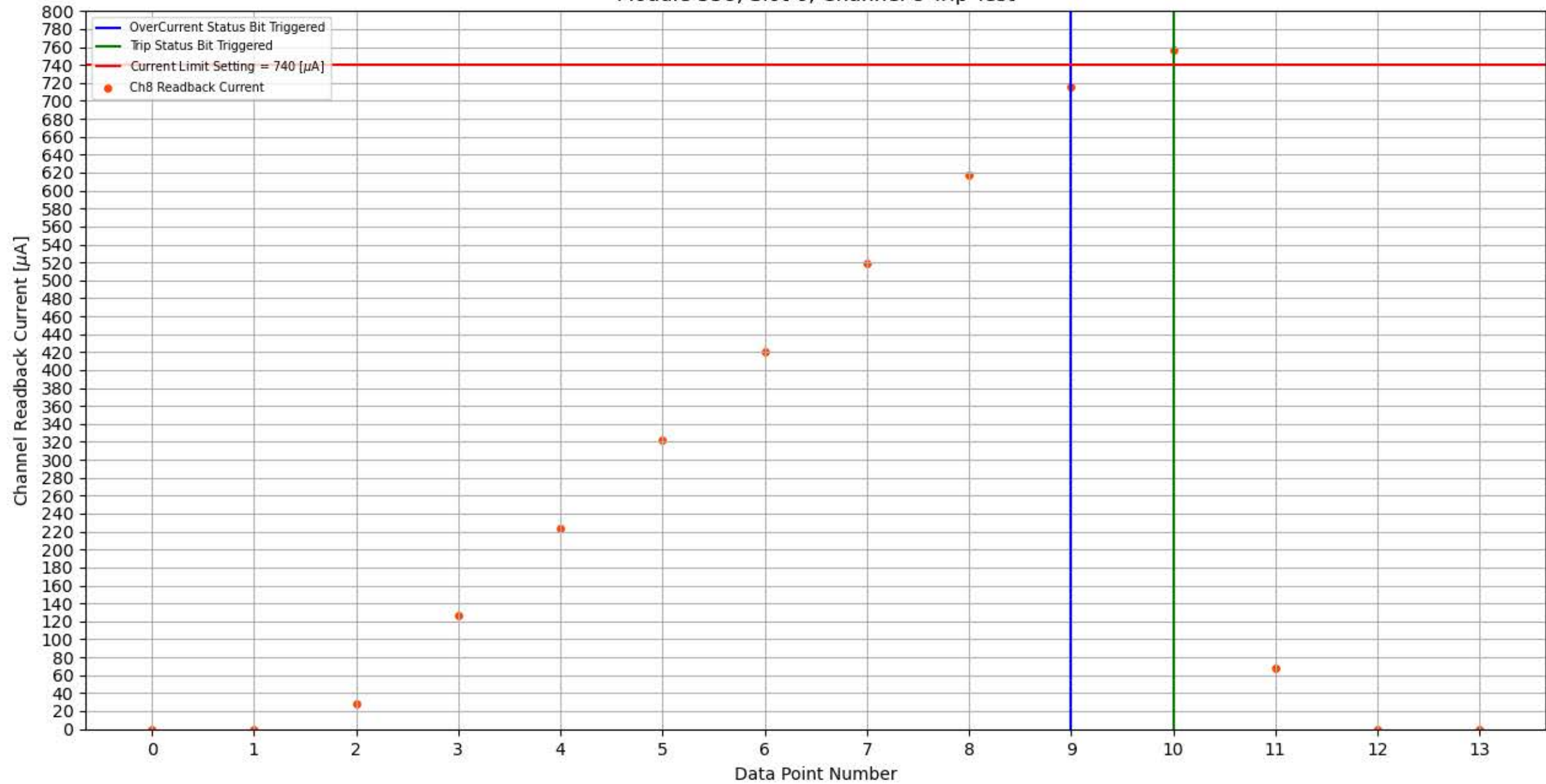
Module 358, Slot 6, Channel 8 Trip Test
