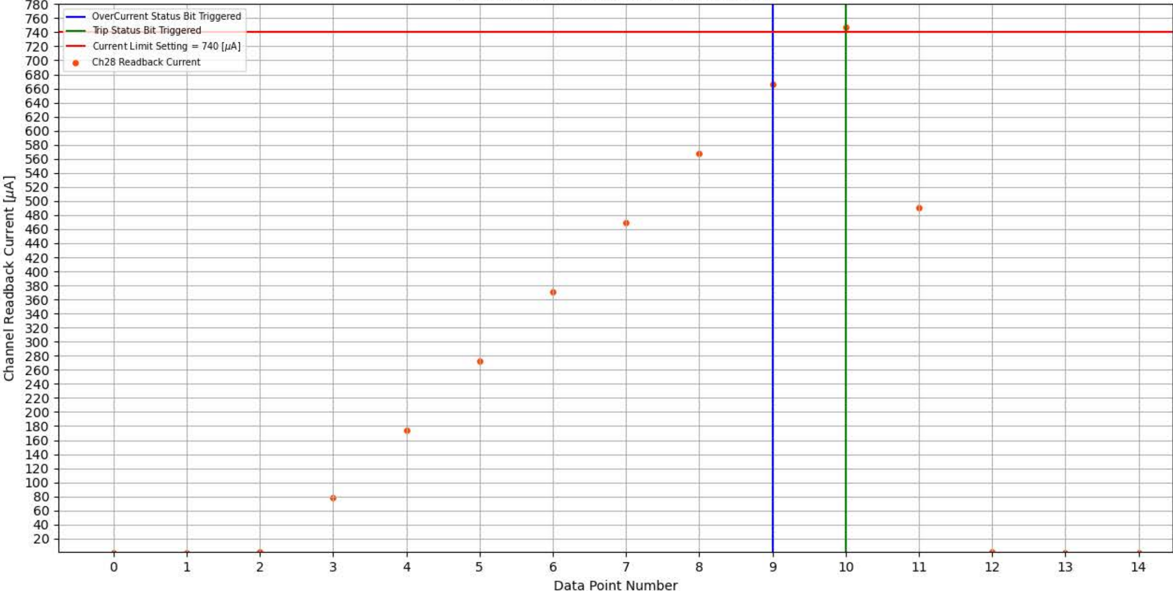
Module 358, Slot 6, Channel 28 Trip Test
