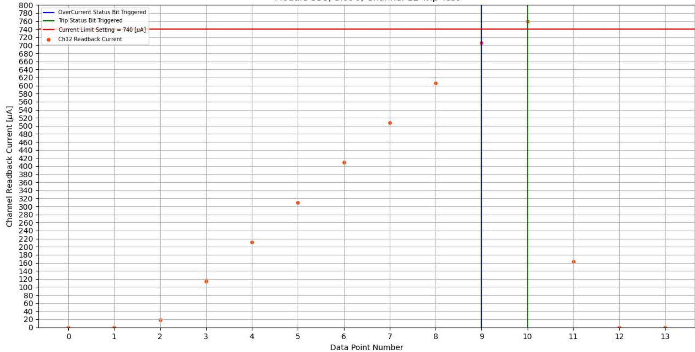
Module 358, Slot 6, Channel 12 Trip Test
