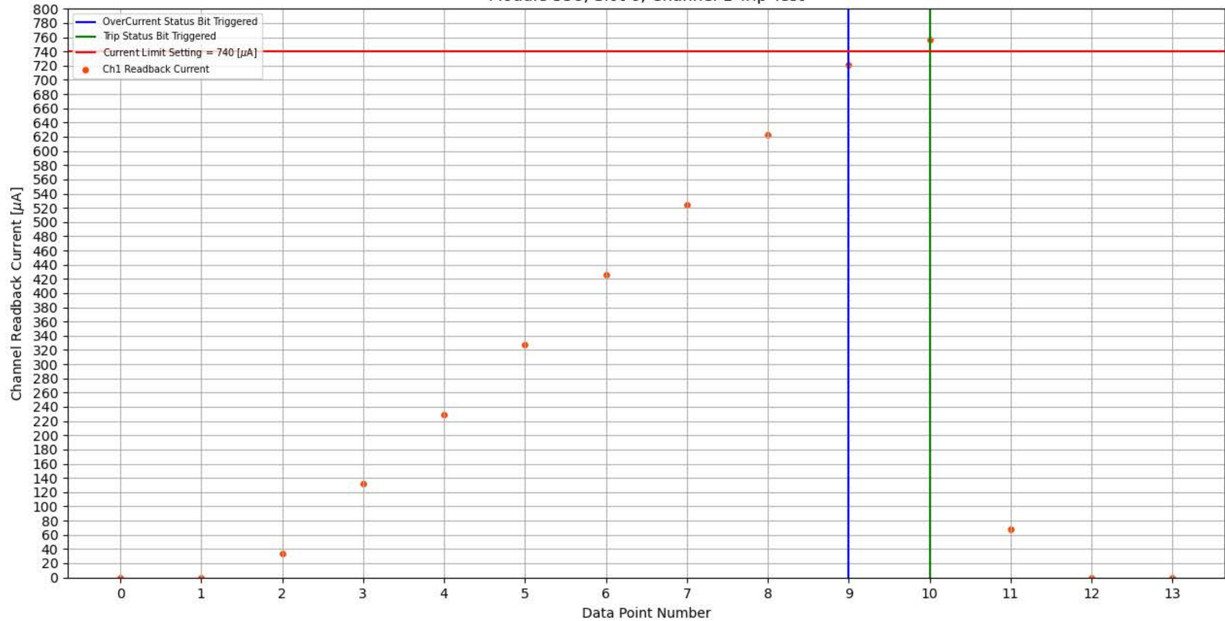
Module 358, Slot 6, Channel 1 Trip Test
