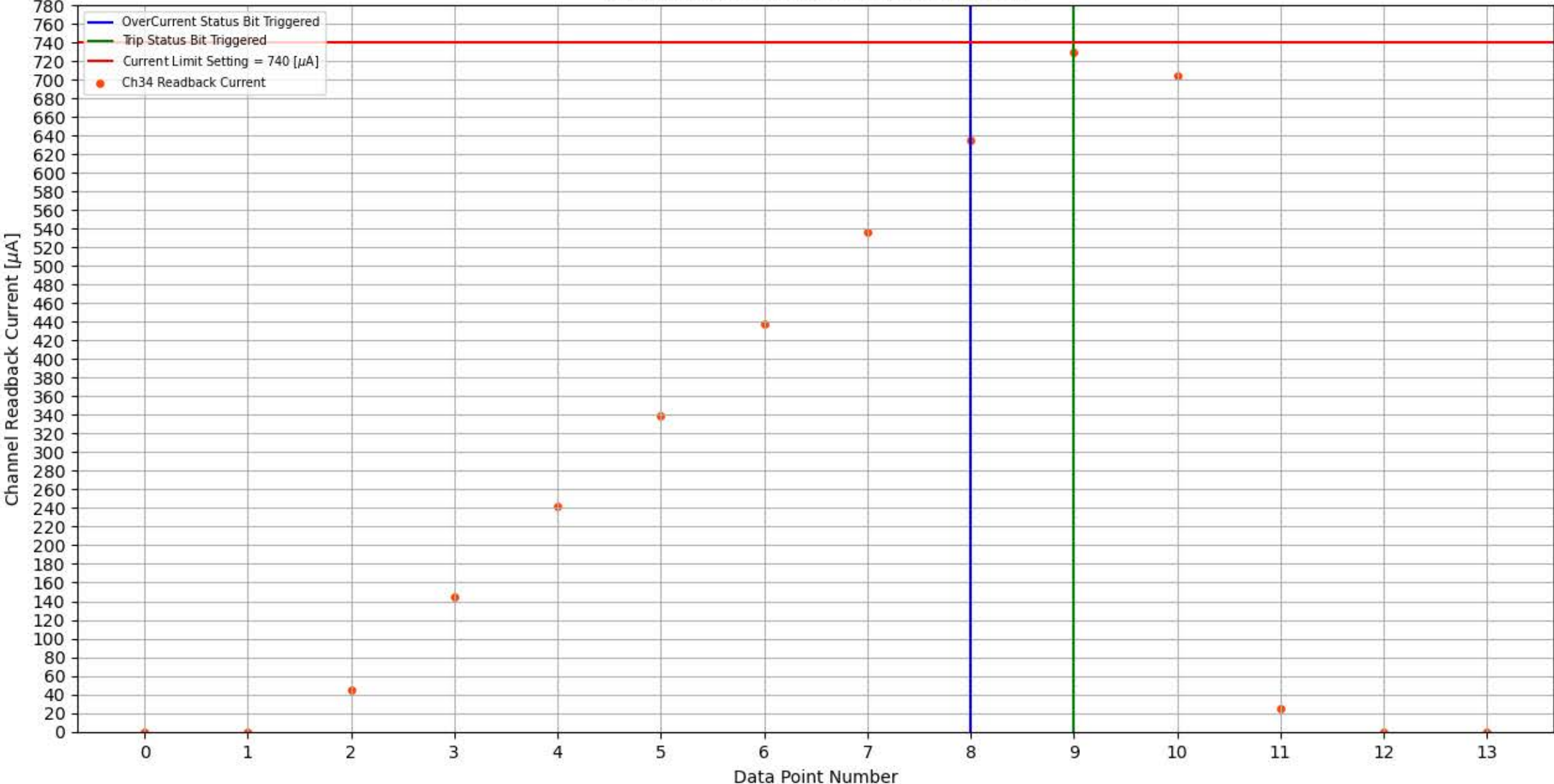
Module 358, Slot 6, Channel 34 Trip Test
