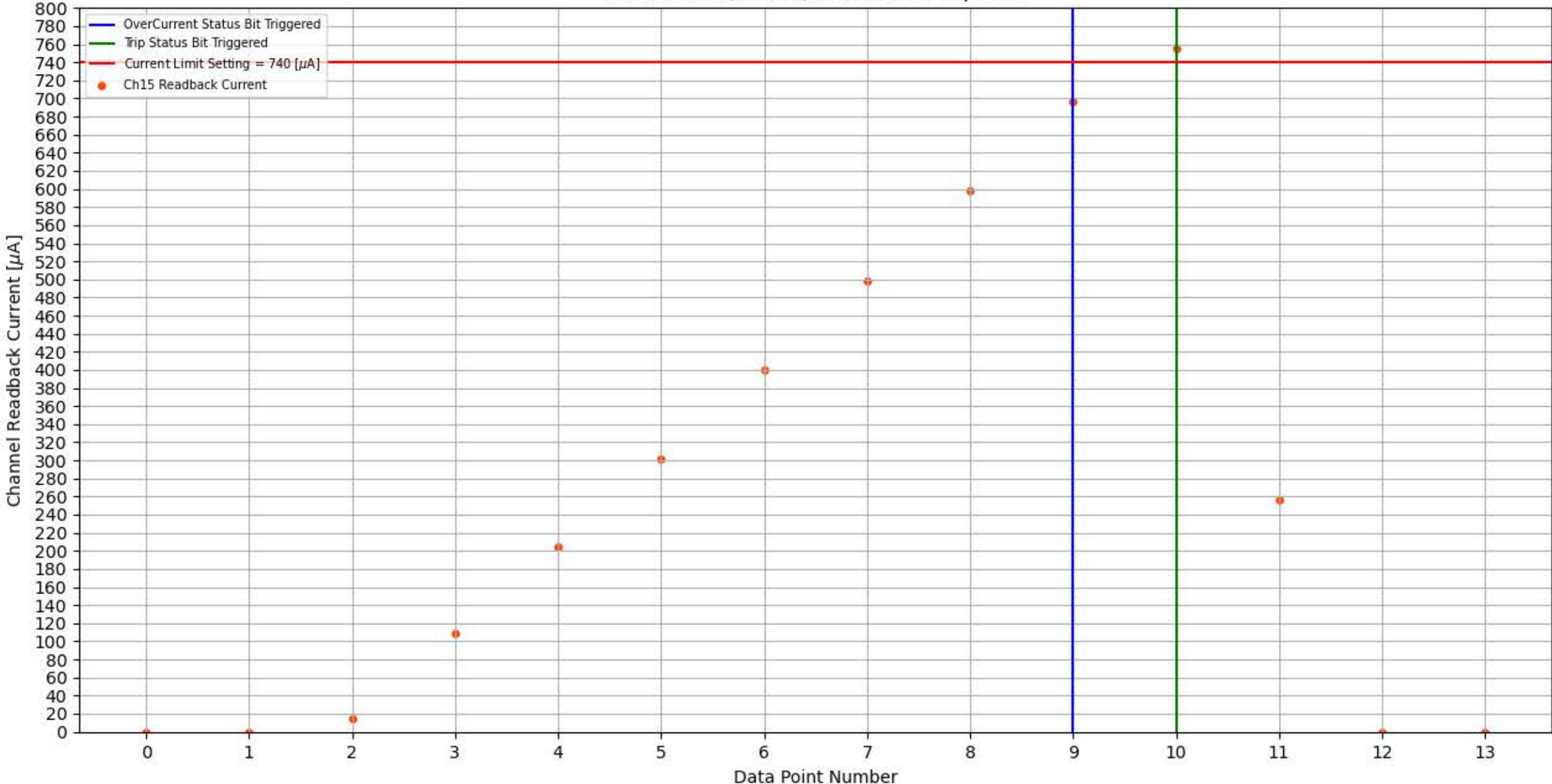
Module 358, Slot 6, Channel 15 Trip Test
