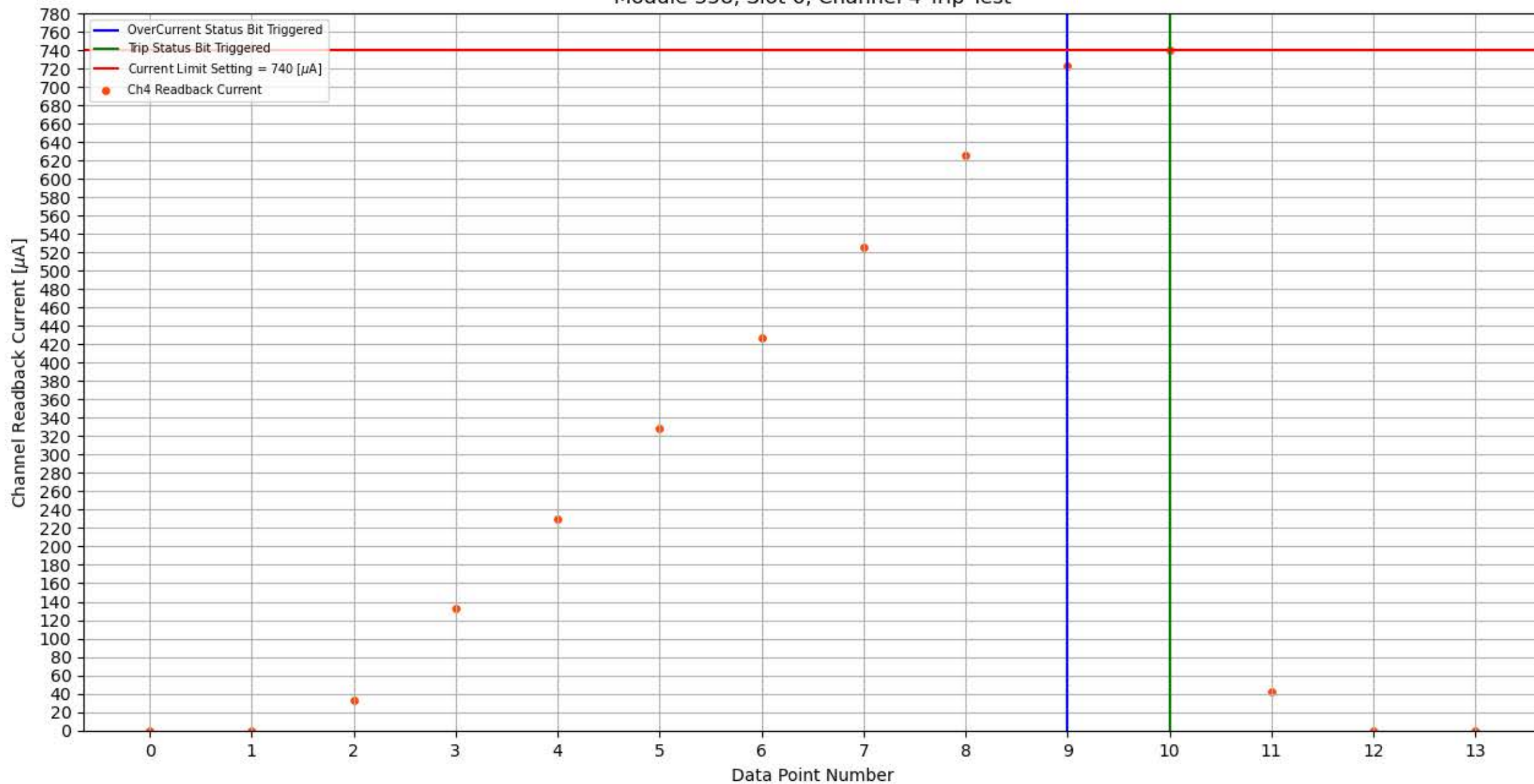
Module 358, Slot 6, Channel 4 Trip Test
