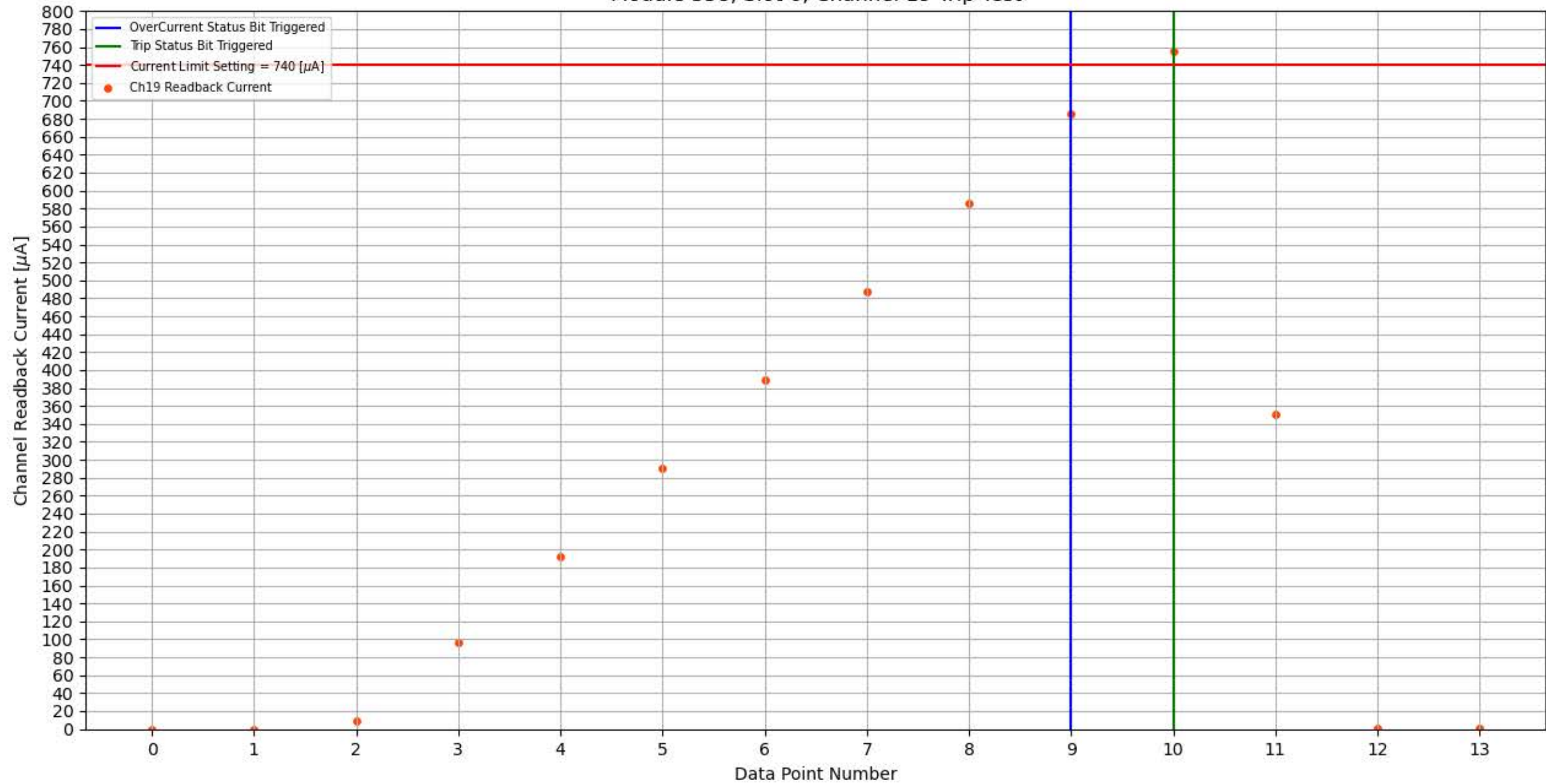
Module 358, Slot 6, Channel 19 Trip Test
