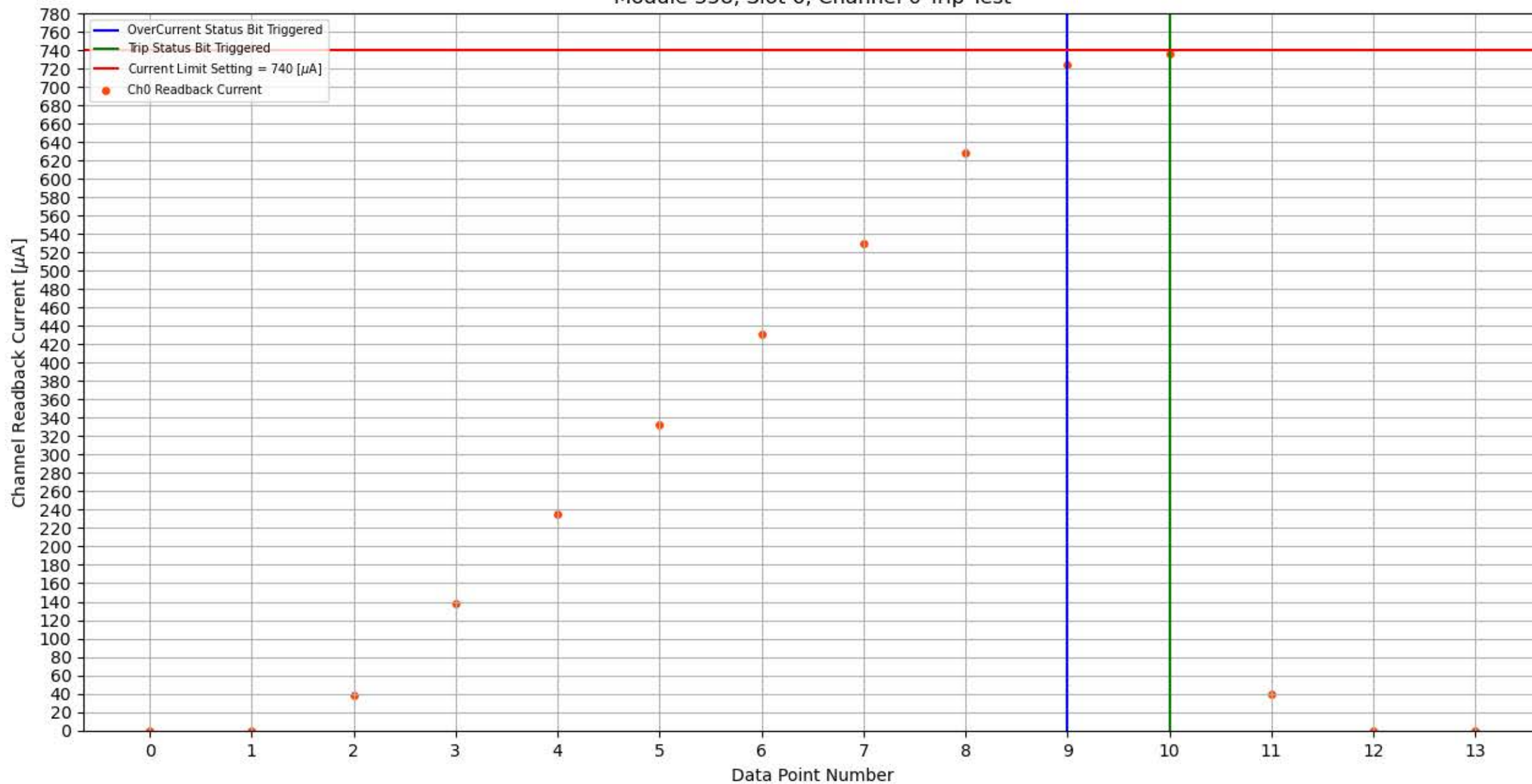
Module 358, Slot 6, Channel 0 Trip Test
