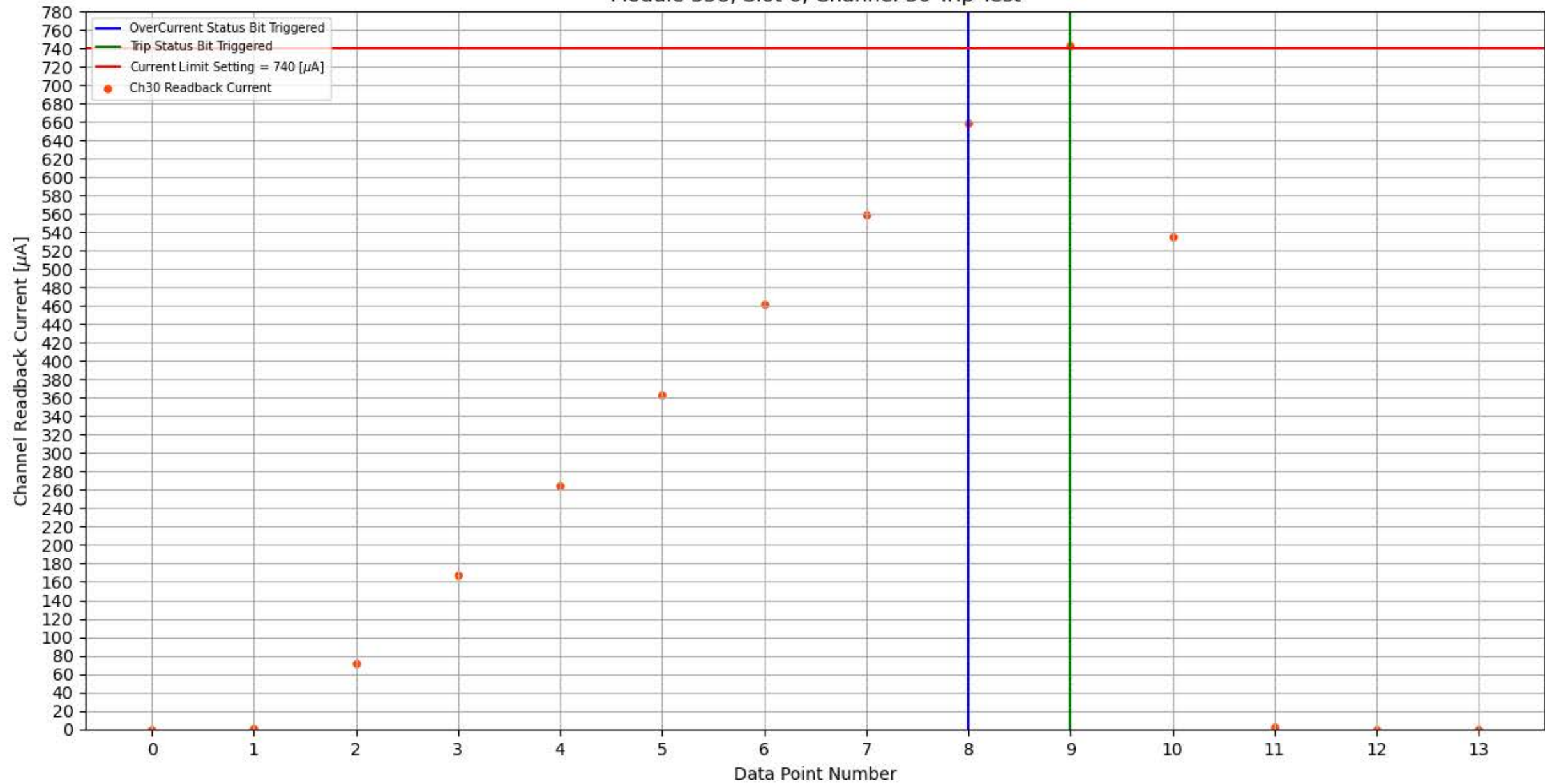
Module 358, Slot 6, Channel 30 Trip Test
