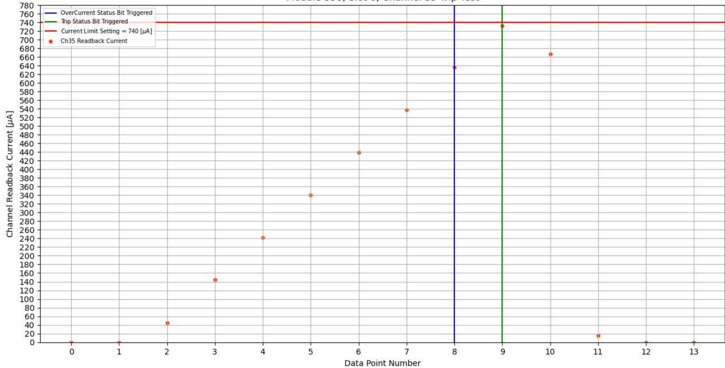
Module 358, Slot 6, Channel 35 Trip Test
