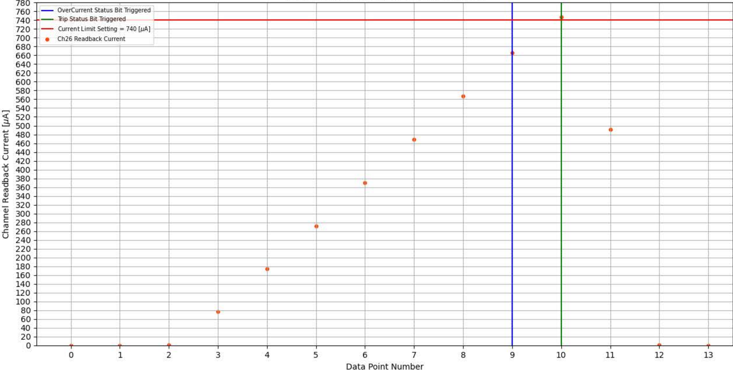
Module 358, Slot 6, Channel 26 Trip Test
