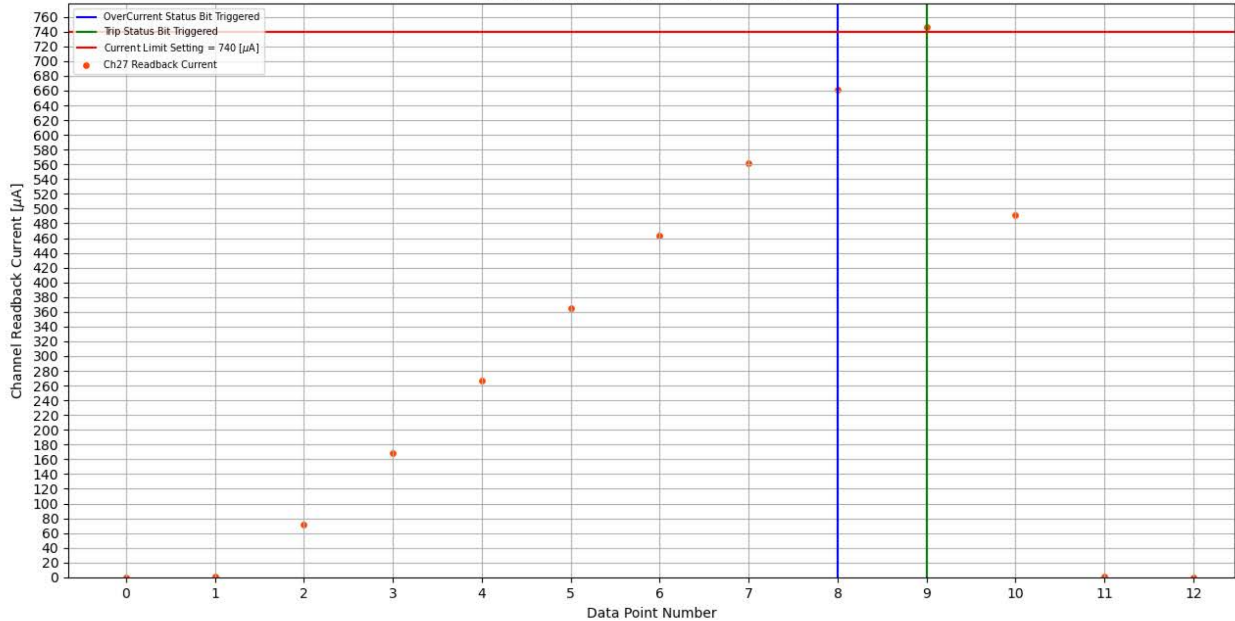
Module 358, Slot 6, Channel 27 Trip Test
