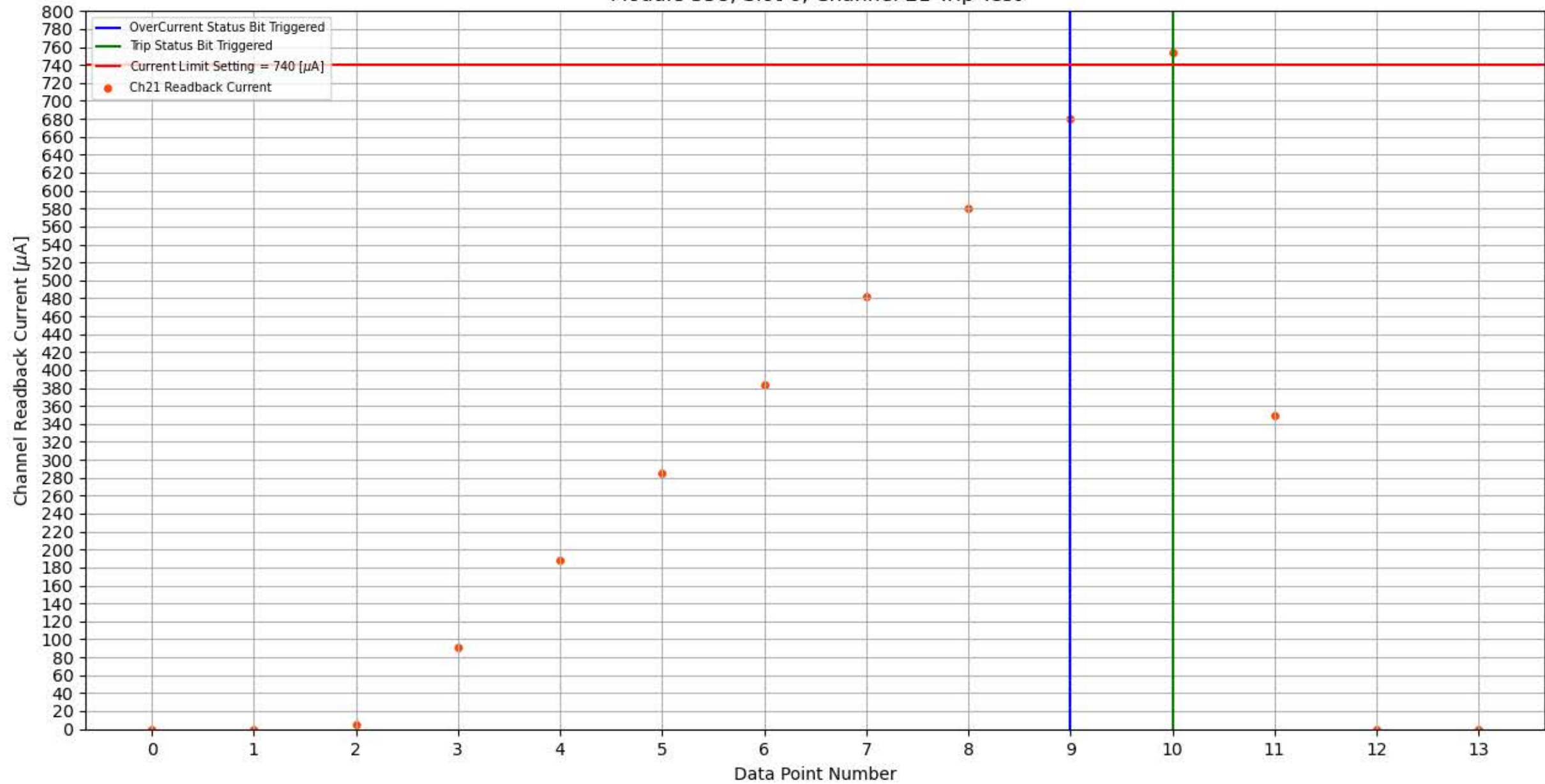
Module 358, Slot 6, Channel 21 Trip Test
