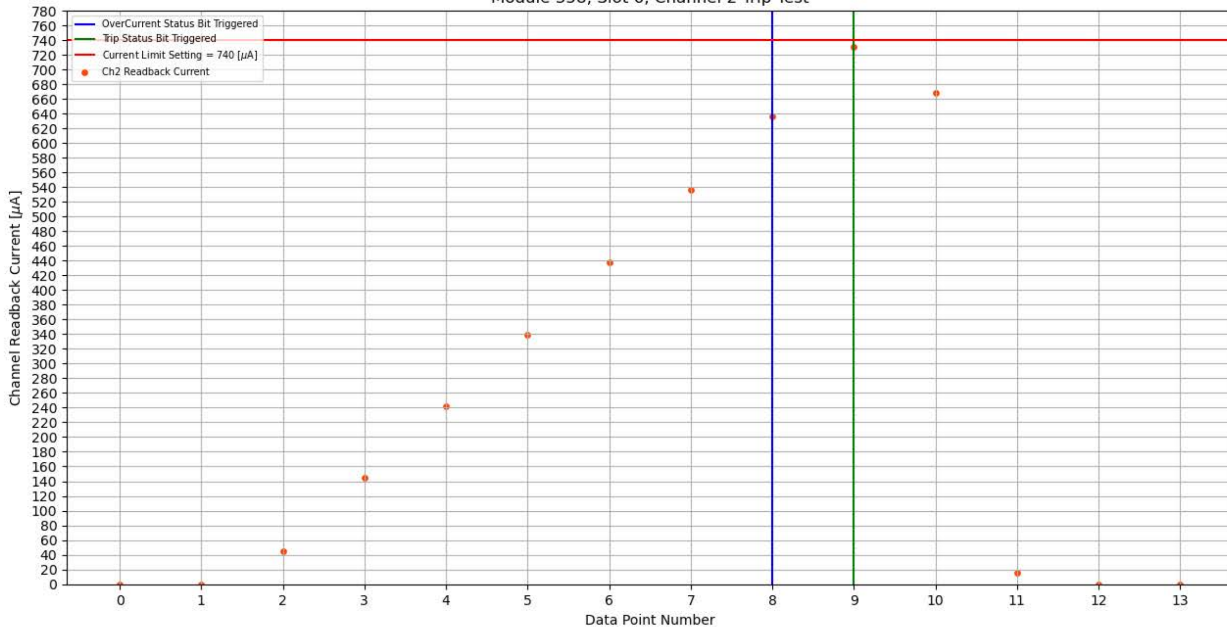
Module 358, Slot 6, Channel 2 Trip Test
