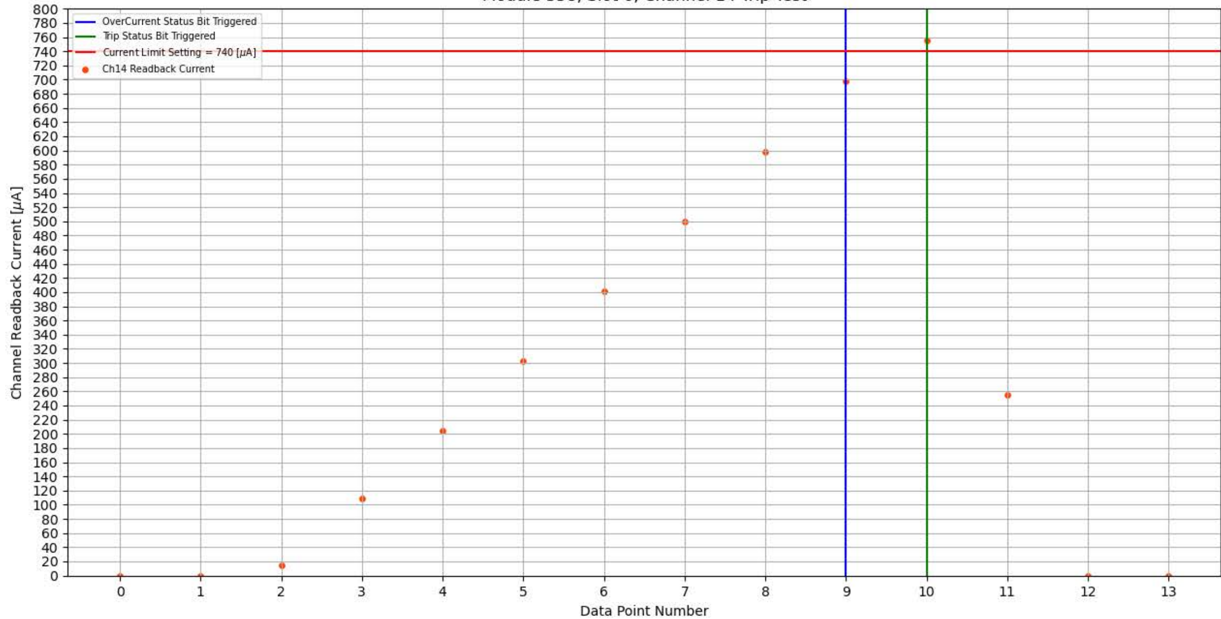
Module 358, Slot 6, Channel 14 Trip Test
