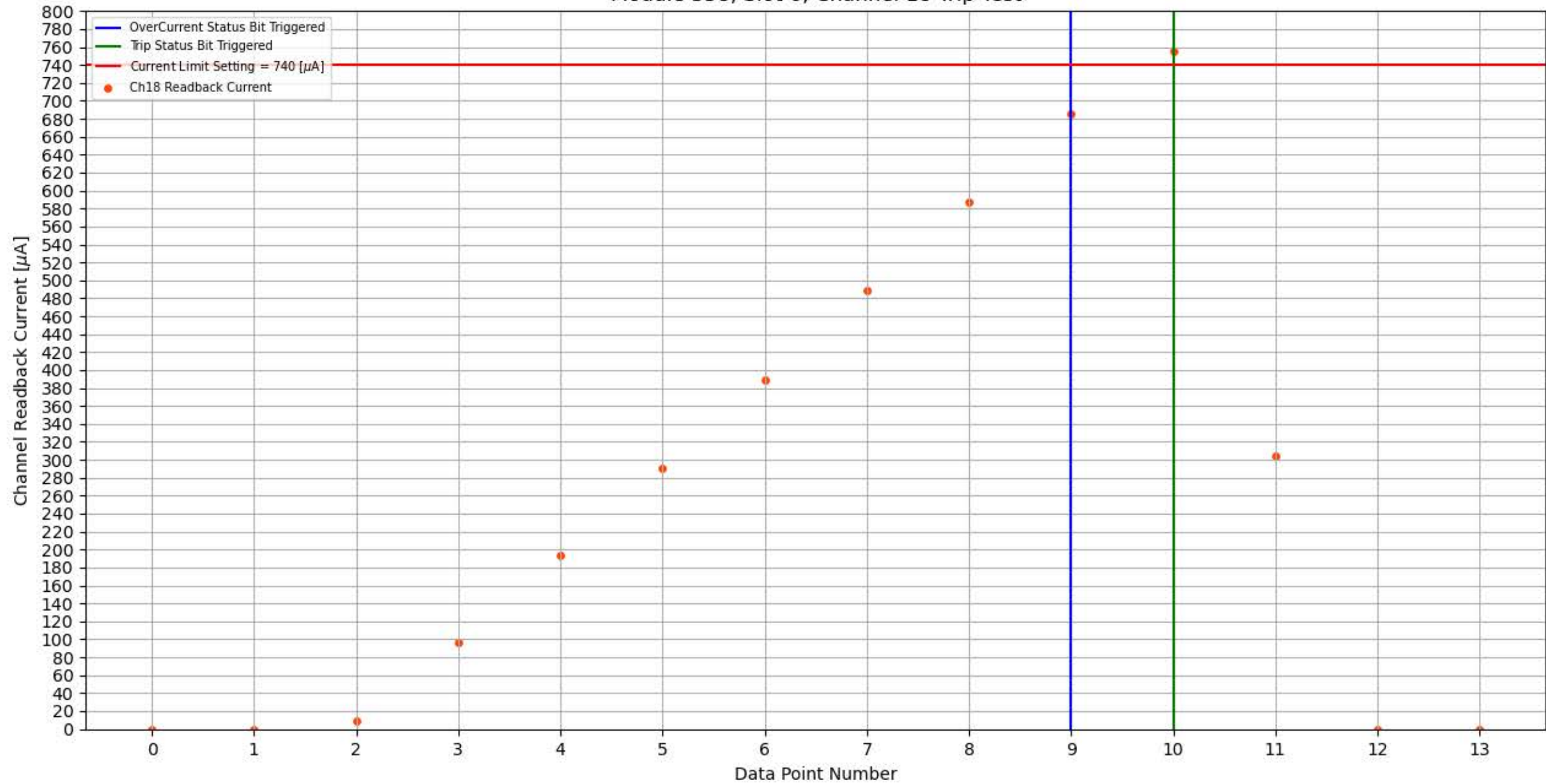
Module 358, Slot 6, Channel 18 Trip Test
