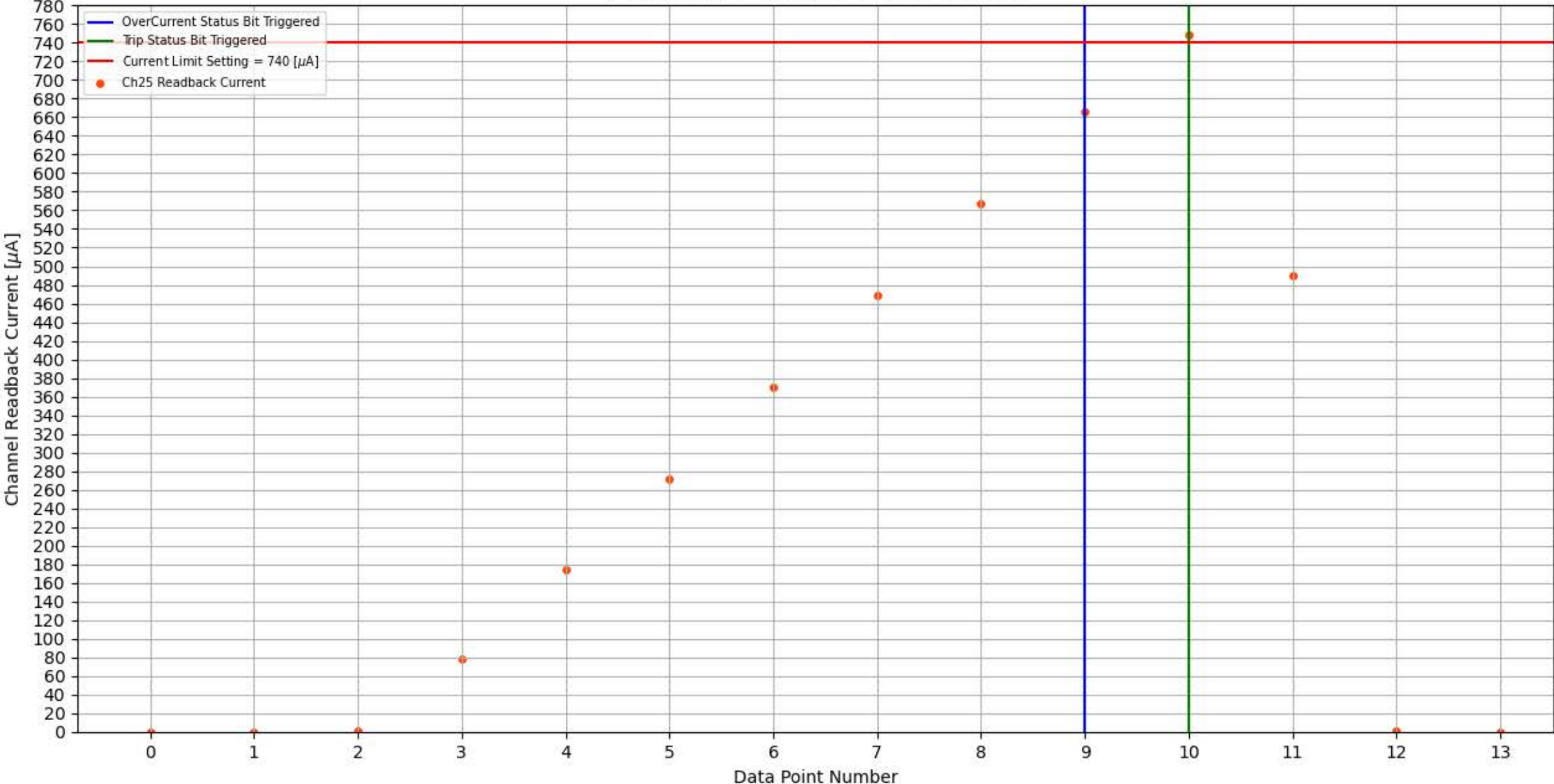
Module 358, Slot 6, Channel 25 Trip Test
