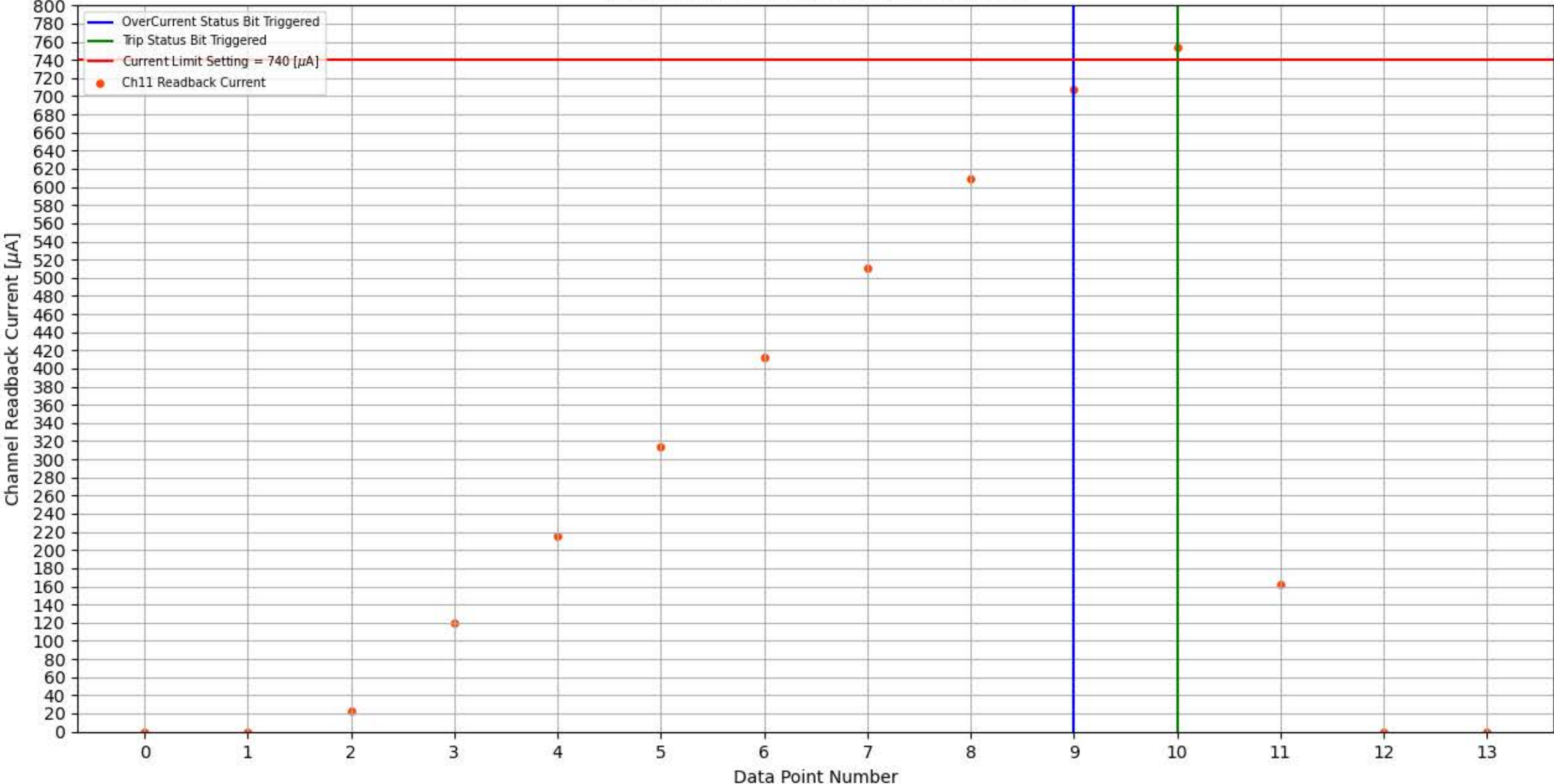
Module 358, Slot 6, Channel 11 Trip Test
