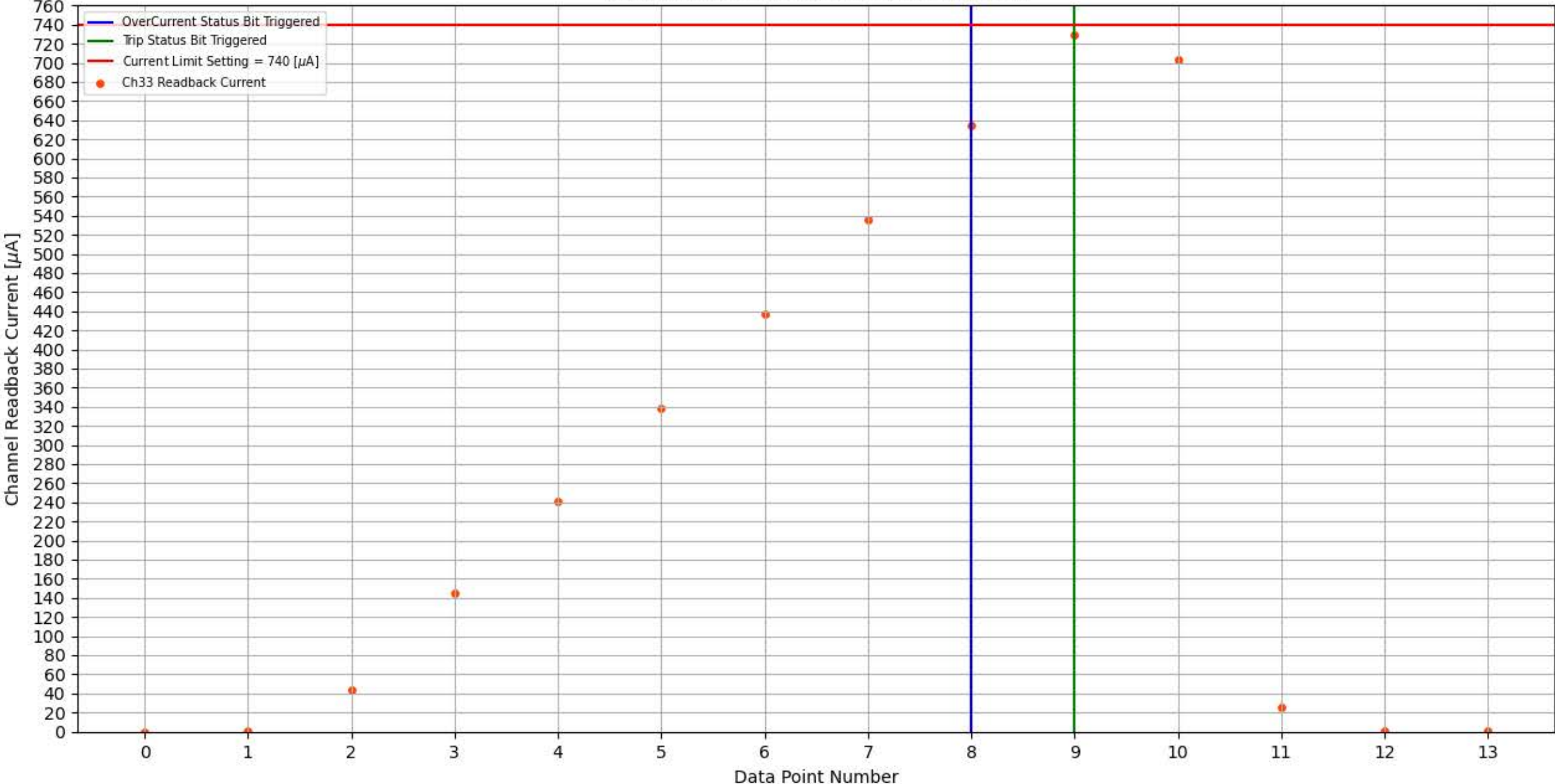
Module 358, Slot 6, Channel 33 Trip Test
