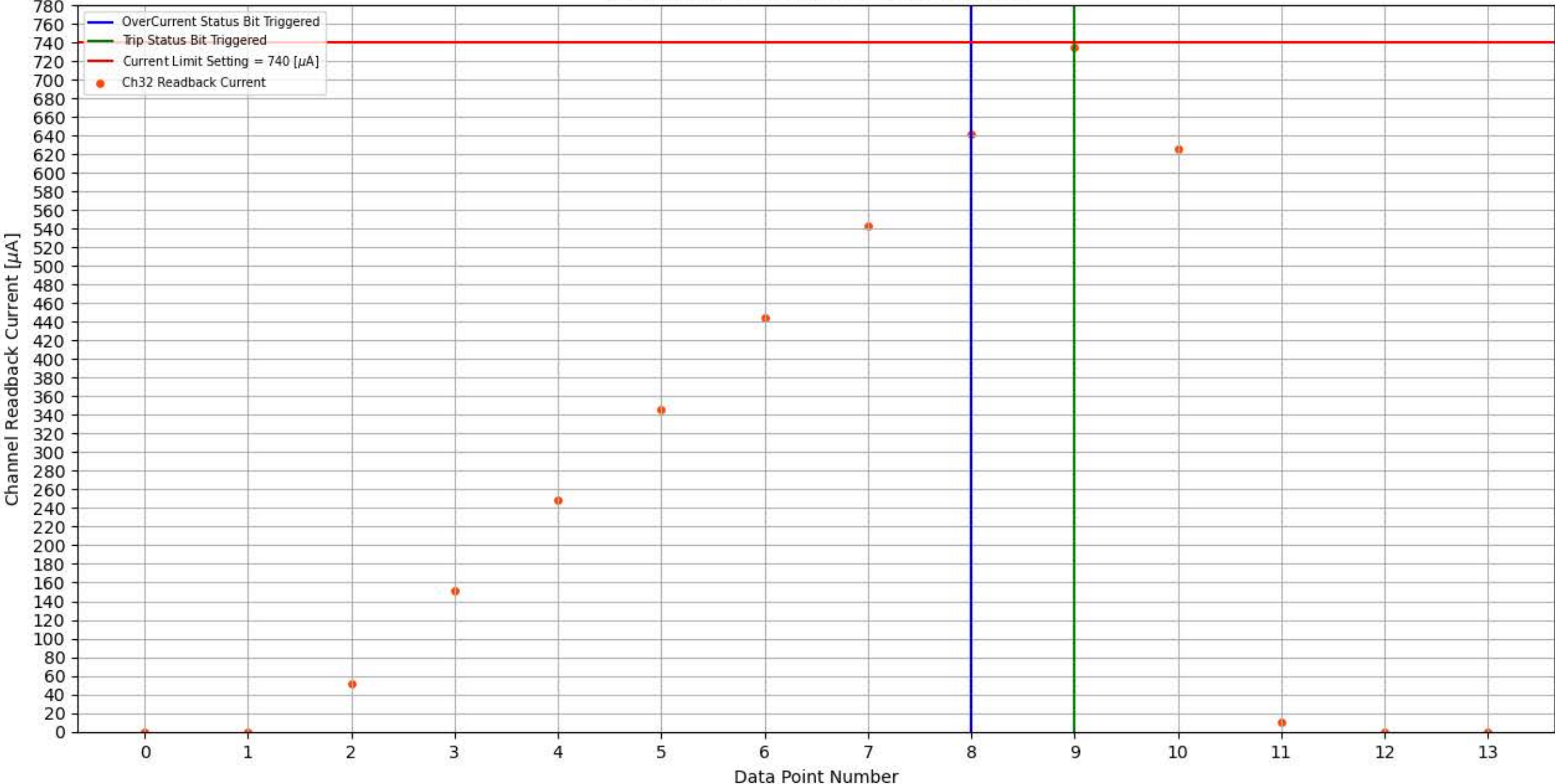
Module 358, Slot 6, Channel 32 Trip Test
