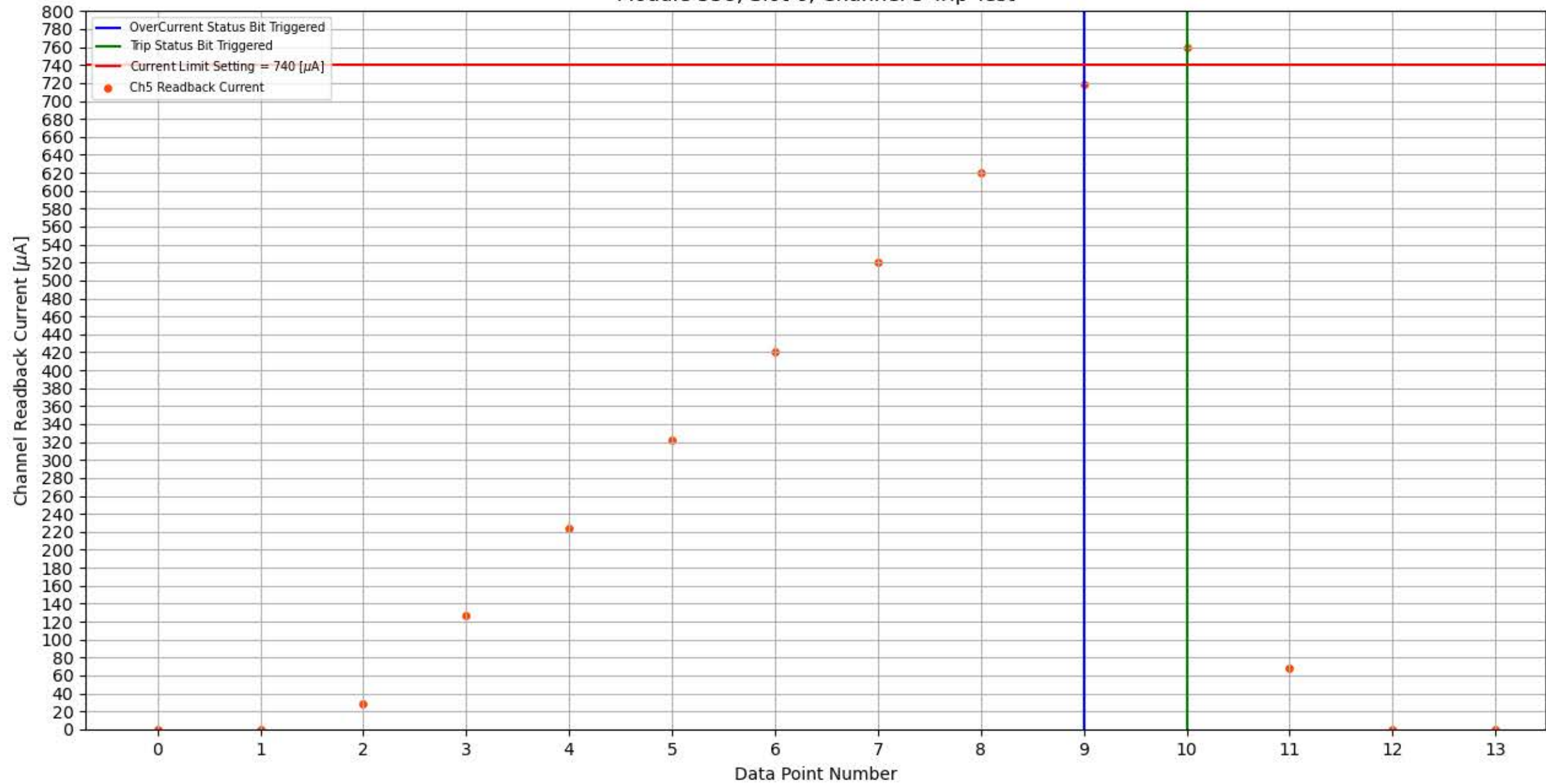
Module 358, Slot 6, Channel 5 Trip Test
