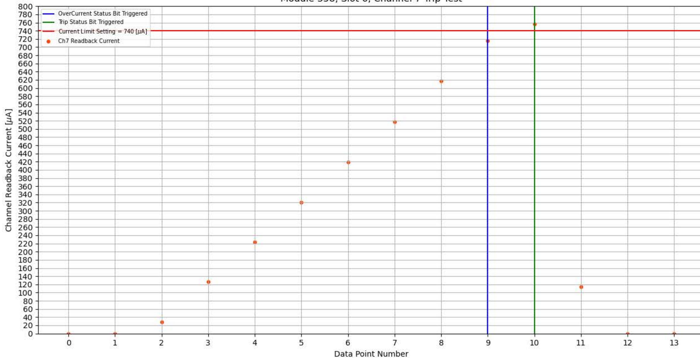
Module 358, Slot 6, Channel 7 Trip Test
