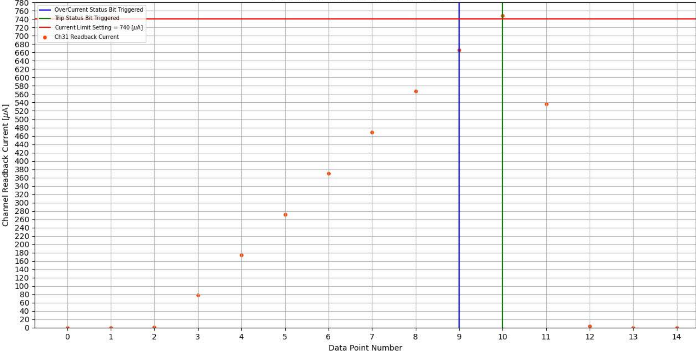
Module 358, Slot 6, Channel 31 Trip Test
