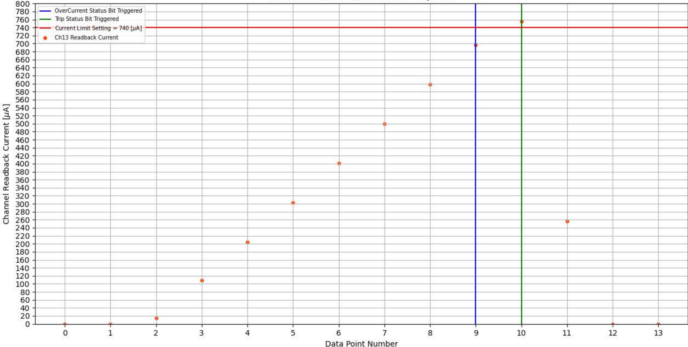
Module 358, Slot 6, Channel 13 Trip Test
