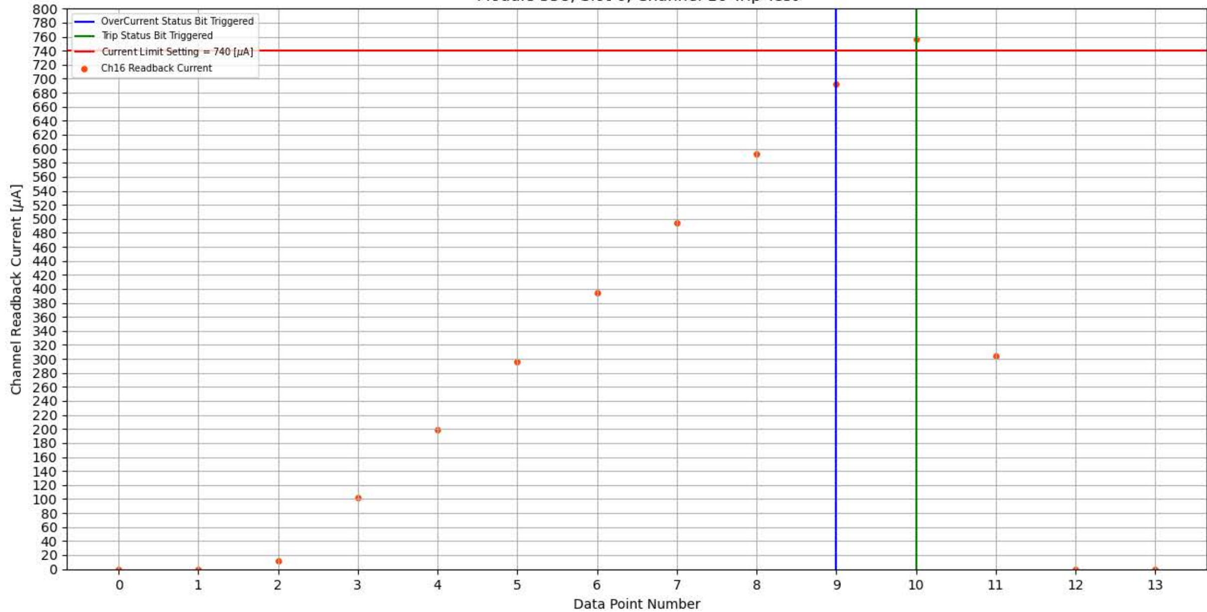
Module 358, Slot 6, Channel 16 Trip Test
