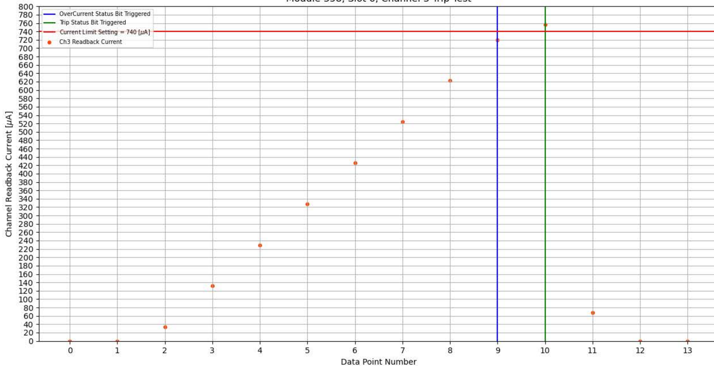
Module 358, Slot 6, Channel 3 Trip Test
