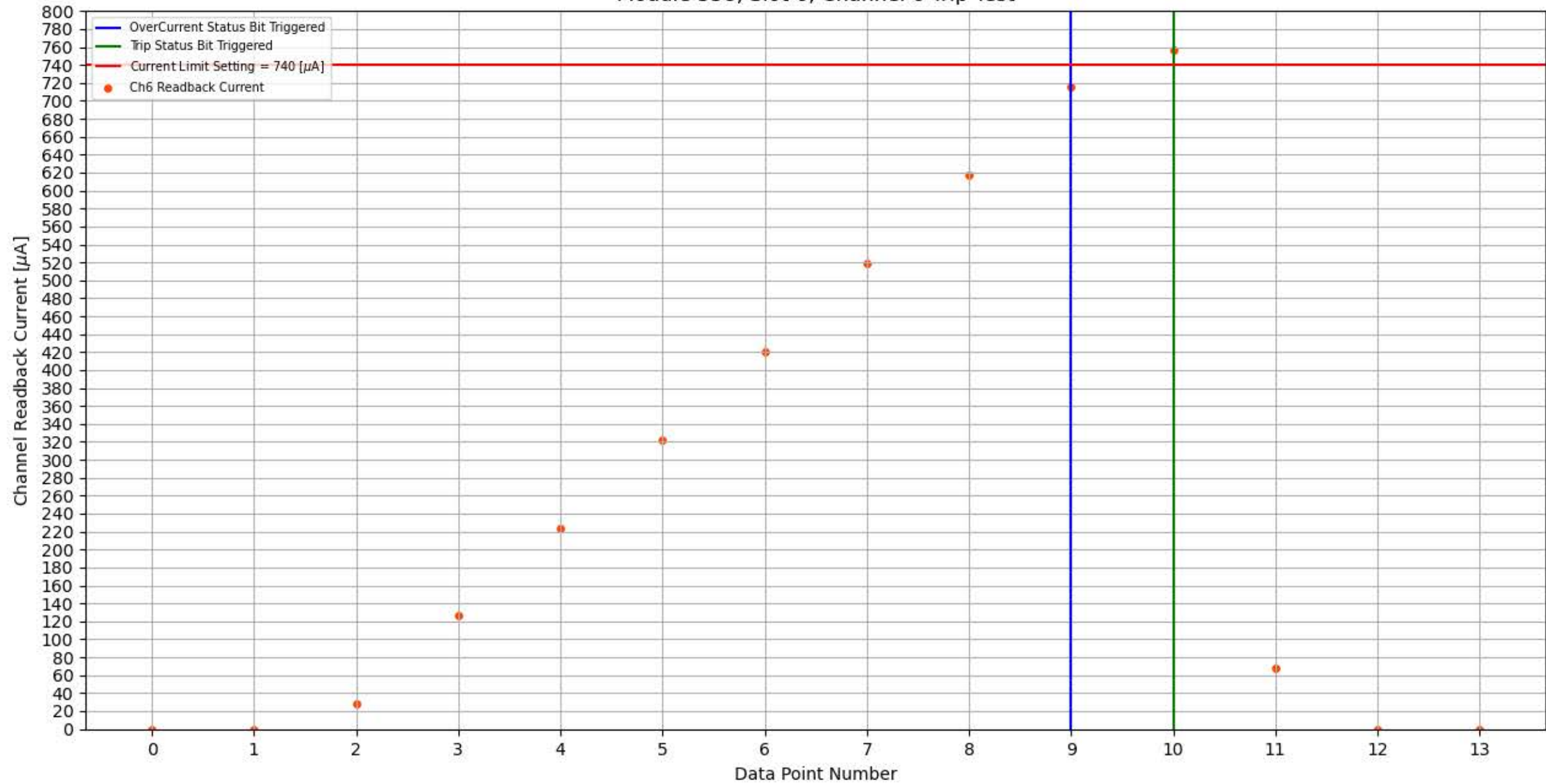
Module 358, Slot 6, Channel 6 Trip Test
