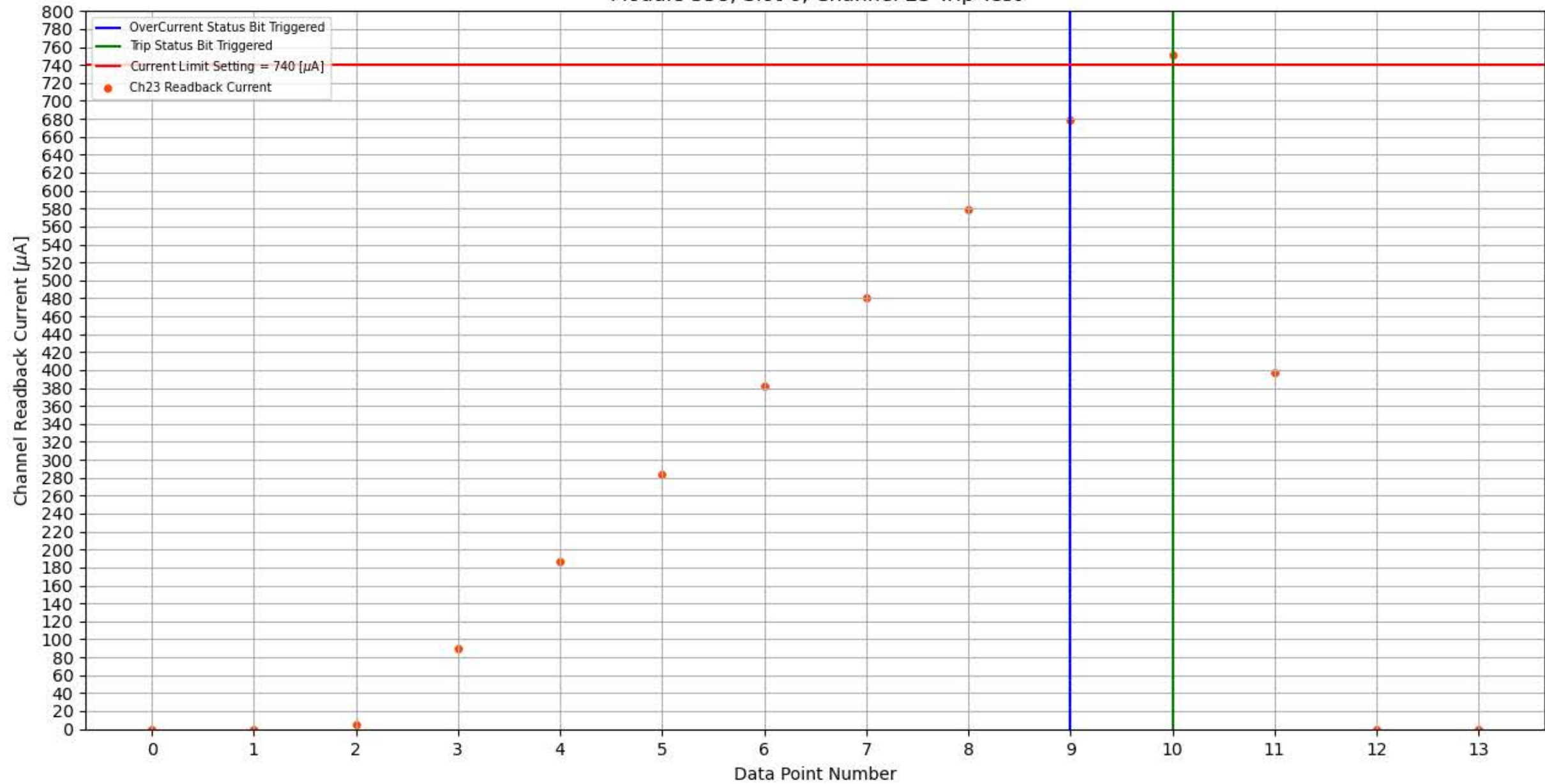
Module 358, Slot 6, Channel 23 Trip Test
