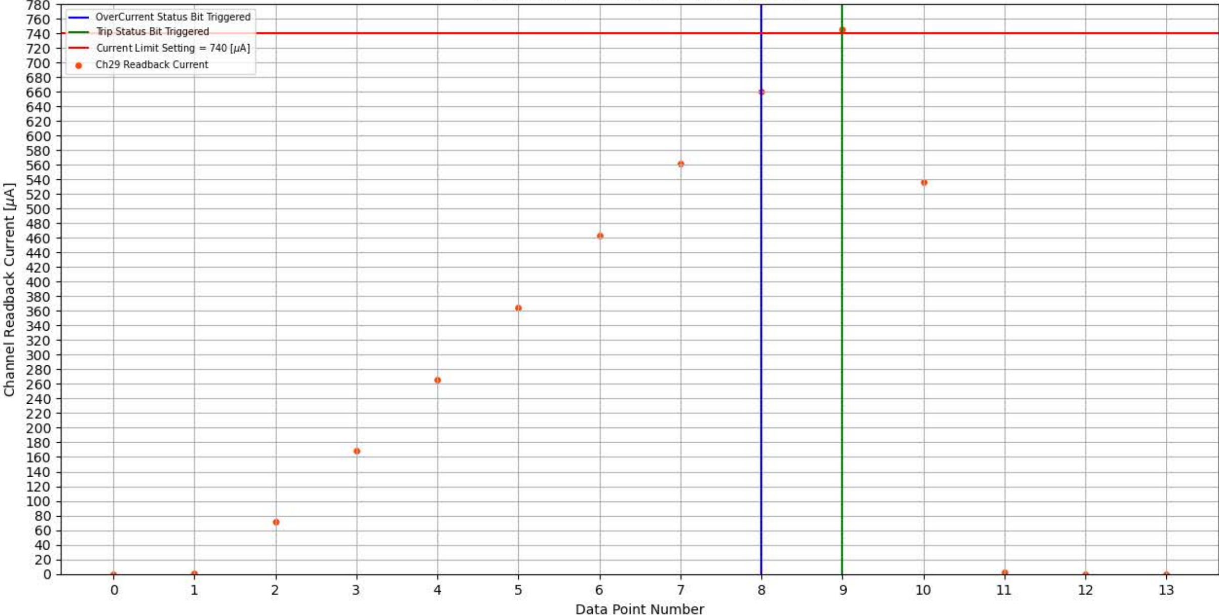
Module 358, Slot 6, Channel 29 Trip Test
