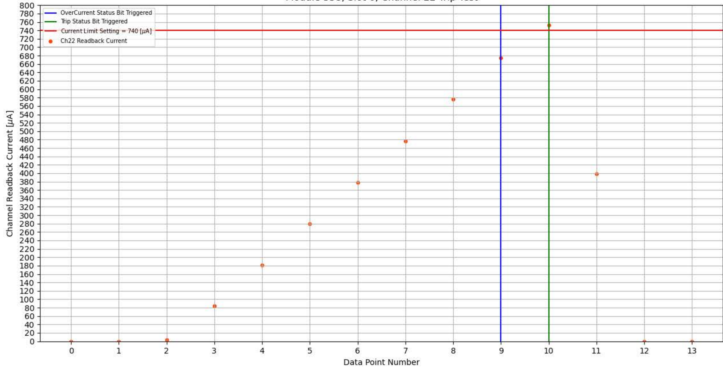
Module 358, Slot 6, Channel 22 Trip Test
