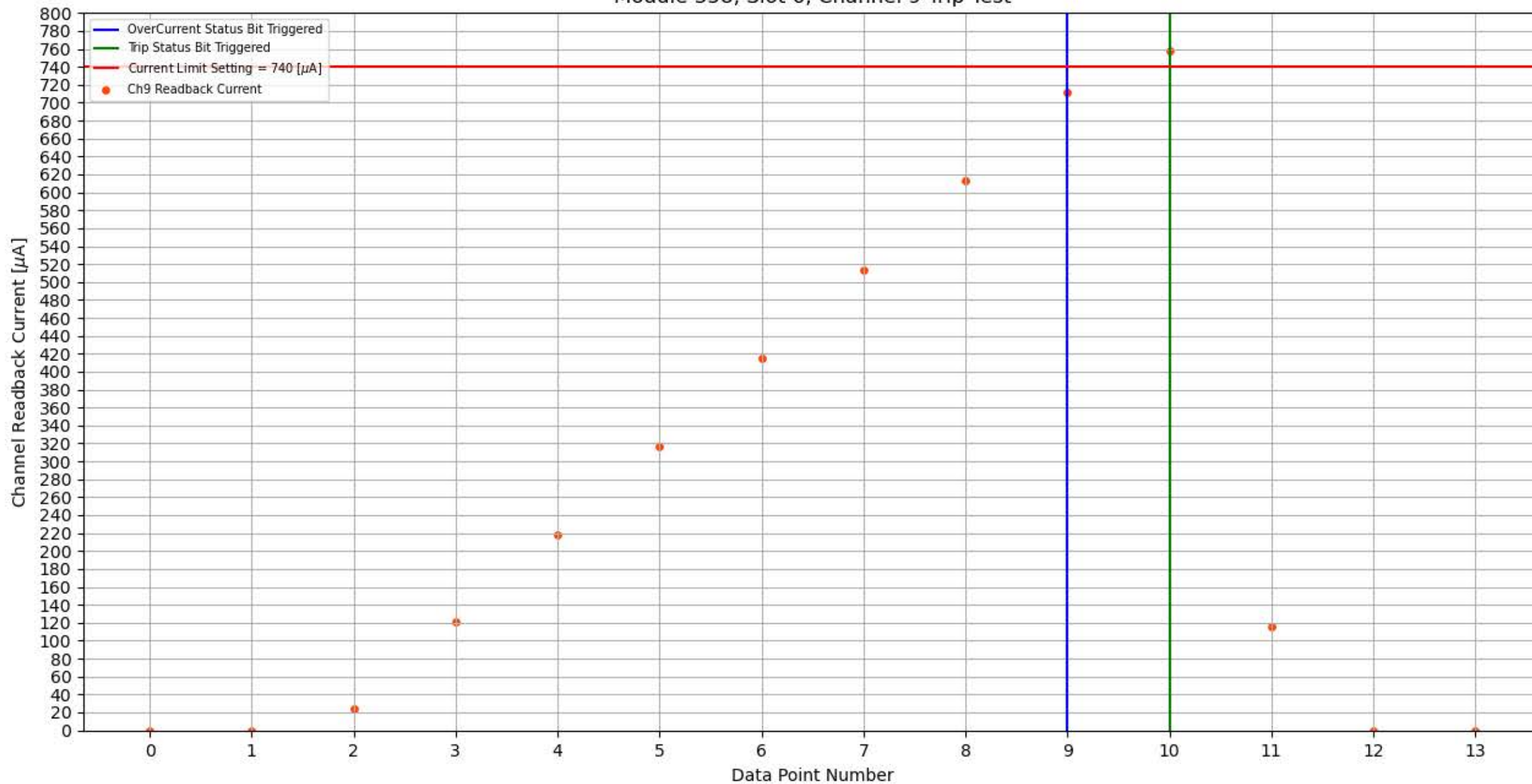
Module 358, Slot 6, Channel 9 Trip Test
