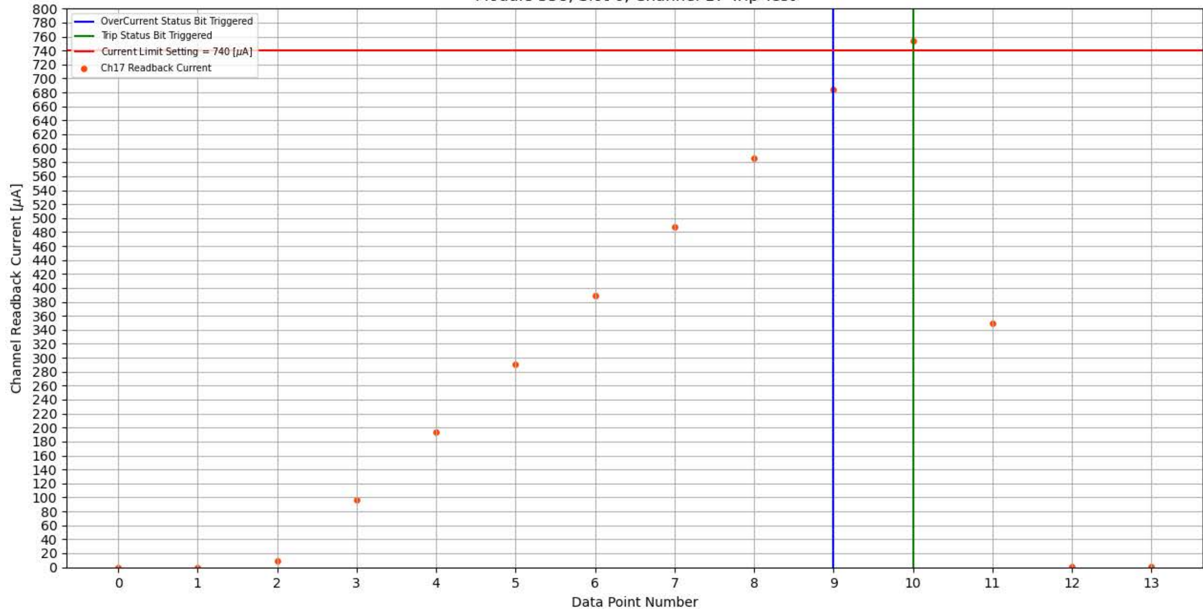
Module 358, Slot 6, Channel 17 Trip Test
