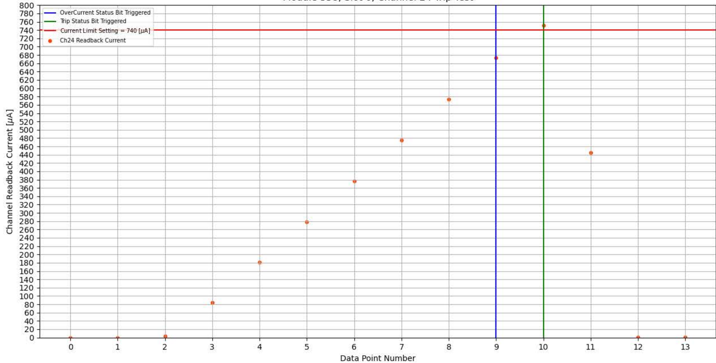
Module 358, Slot 6, Channel 24 Trip Test
