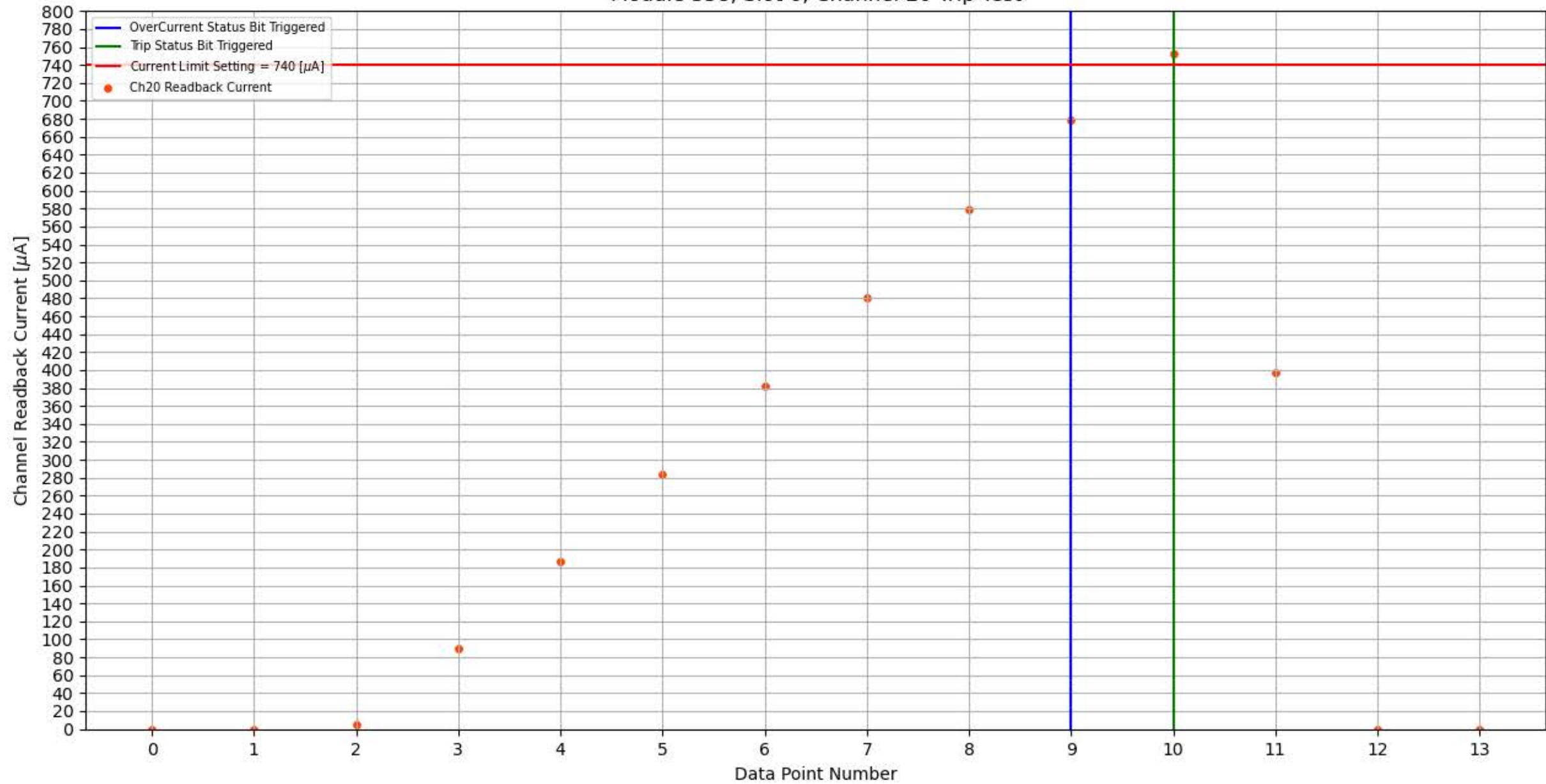
Module 358, Slot 6, Channel 20 Trip Test
